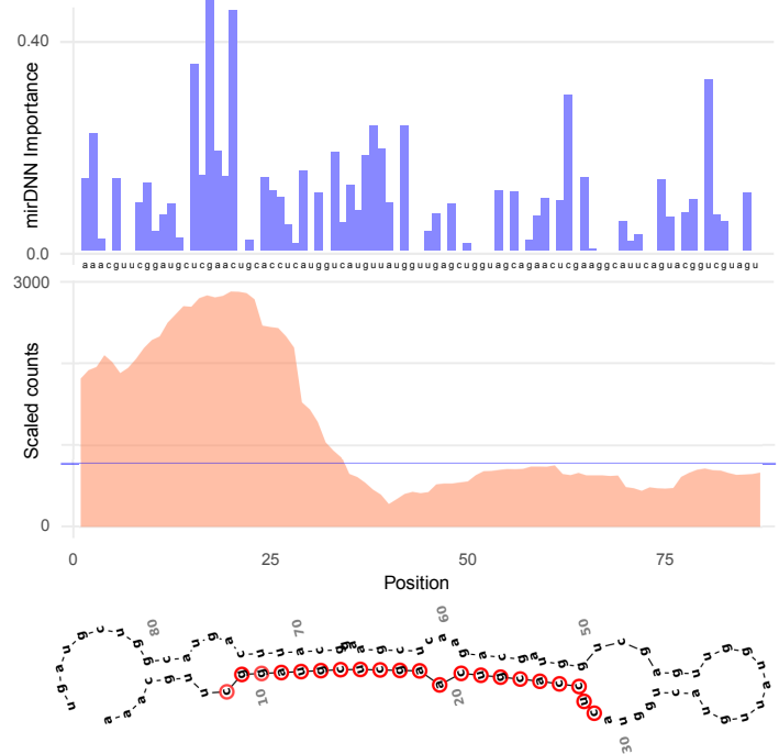
Figure 4: Interpretable prediction of the sars_cov2_101-701_stem-379-465 candidate sequence to pre-miRNA in SARS-CoV-2. (top) Importance given by mirDNN to each nucleotide in the sequence. (middle) Experimental reads for this sequence, average of two replicates of the biological experiment. Horizontal blue line indicating the average reads count for the complete genome. (bottom) Corresponding secondary structure predicted using RNAfold, with the mature miRNA marked in red.
