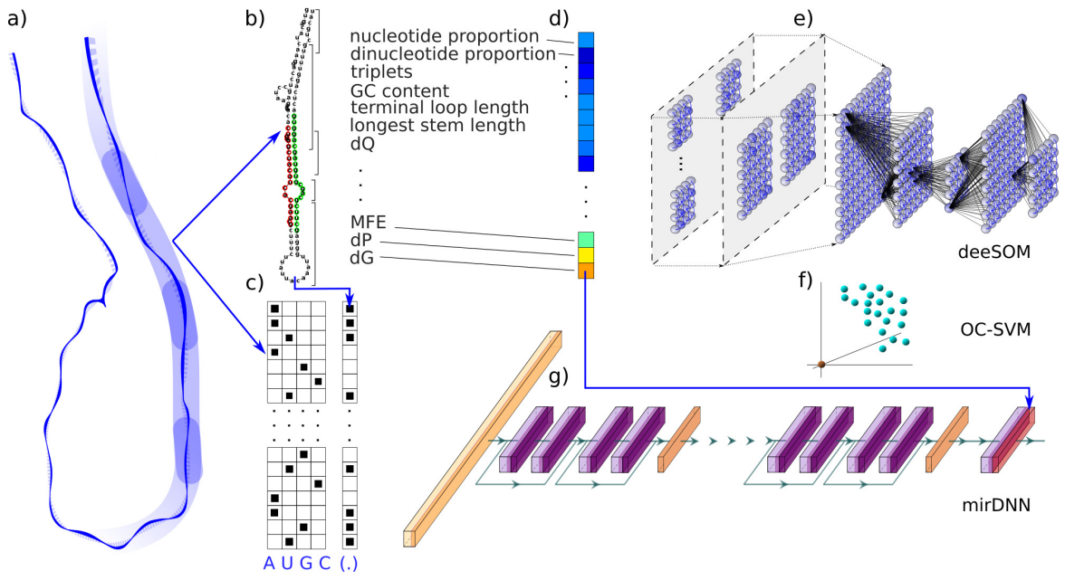
Figure 1: Processing pipeline based in machine learning for finding potential pre-miRNAs in the genome of the Severe Acute Respiratory Syndrome-Coronavirus 2 (SARS-CoV-2), responsible for the novel coronavirus disease (COVID-19): a) Genome cut into sequences, b) Prediction of secondary structure and feature extraction, c) One-hot encoding of the nucleotides (A, U, G, C) and matches (‘(’) or mismatches (‘.’) in the secondary structure, d) Input feature vector, e) The deeSOM classifier, f) The OC-SVM classifier, g) The mirDNN model.
