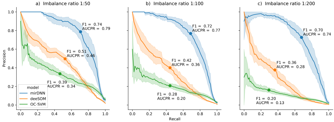
Figure 2: Precision-recall curves for each model and imbalance ratio a) 1:50, b) 1:100, c) 1:200. Bold line is the mean value, and the shaded area is its standard deviation from cross-validation results. Maximum F_1 and AUCPR are indicated for each curve.
