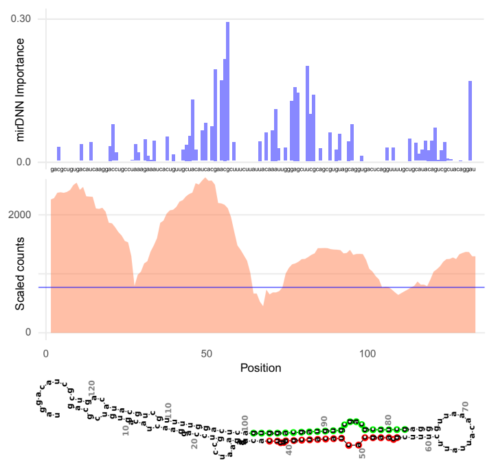
Figure 3: Interpretable prediction of the sars_cov2_26601-27201_stem-392-524 candidate sequence to pre-miRNA in SARS-CoV-2. (top) Importance given by mirDNN to each nucleotide in the sequence. (middle) Experimental reads for this sequence, average of two replicates of the biological experiment. Horizontal blue line indicating the average reads count for the complete genome. (bottom) Corresponding secondary structure predicted using RNAfold, in this case with two possible mature miRNAs marked in red and green, respectively.
