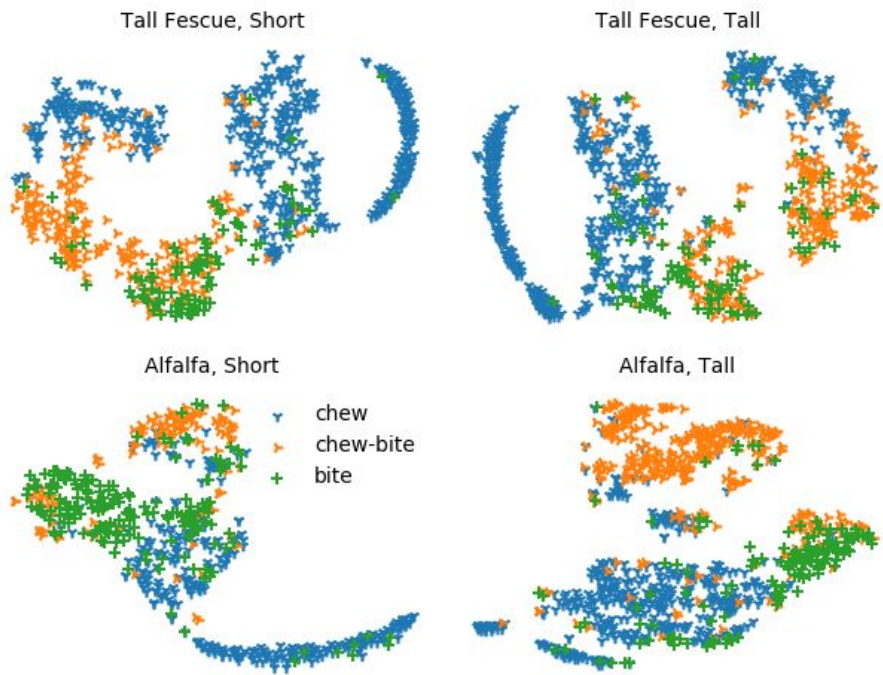
Figure 4: T-distributed stochastic neighbor embedding for datasets per species and height. Each data point corresponds to a jaw movement.
