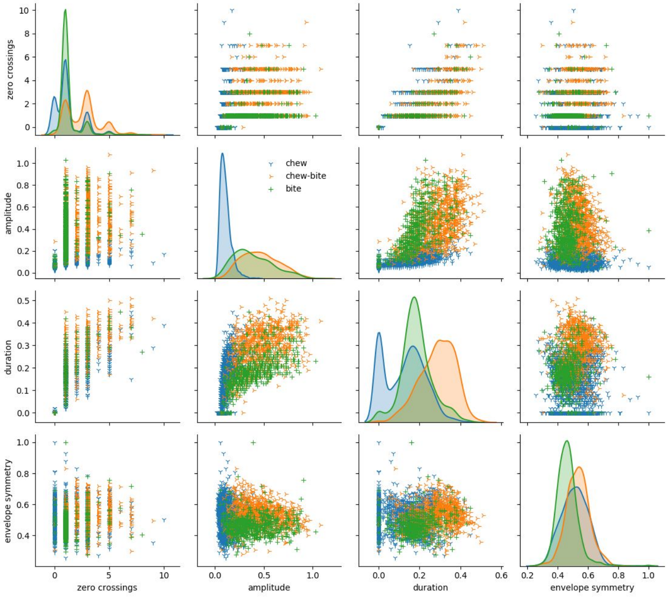
Figure 5: Uni- and bivariate distributions of features for all species and heights by jaw movement type.
