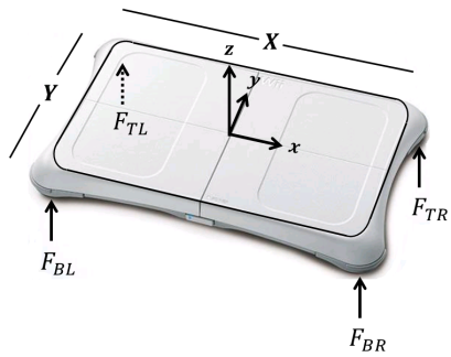
Figura 4. Wii Balance Board En "Validating and Calibrating the Nintendo Wii Balance Board to Derive Reliable Center of Pressure Measures", por Leach, J. M., 2014, https://www.researchgate.net/
