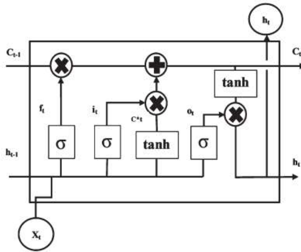
Fig. 1. LSTM unit architecture
