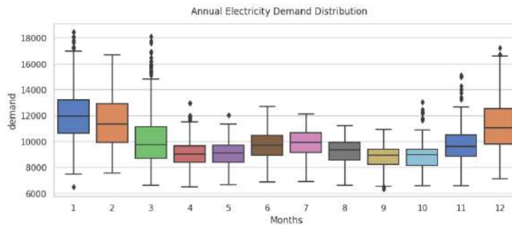
Fig. 3. Annual demand cycle [MWh]
