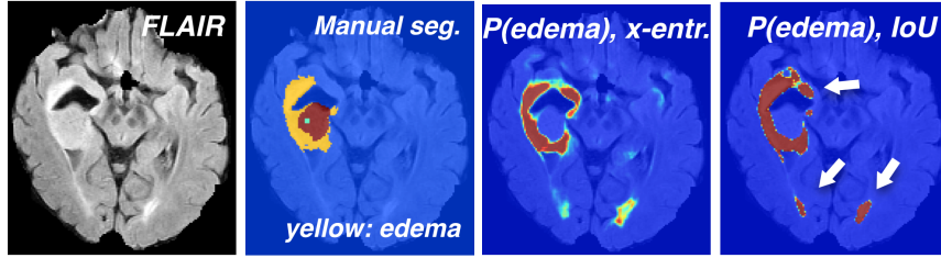
Fig. 1: Left to right: FLAIR; manual annotation of a BRATS’17 subject, where yellow depicts oedema surrounding tumour core; confidence of a CNN predicting oedema, trained with cross-entropy or IoU loss. Although overall performance is similar, training with IoU (or Dice, not shown) loss alters the CNN’s behaviour, which tends to output only highly confident predictions, even when false.
