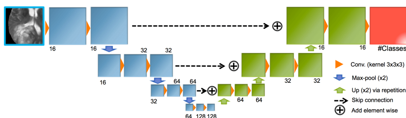
Fig. 5: Schematic of an adapted Unet used in our experiments. Depicted are number of feature maps per layer. All kernels and feature maps are 3D, even though not depicted for simplicity.
