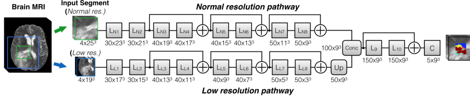
Fig. 3: We used two DeepMedics [13] in our experiments. The smaller of the two is depicted, where the number of feature maps and their dimension at every layer are depicted in the format (Number \times Size) . The second model used in the ensemble is wider, with double the number of feature maps at every layer. All kernels and feature maps are 3D, even though not depicted for simplicity.
