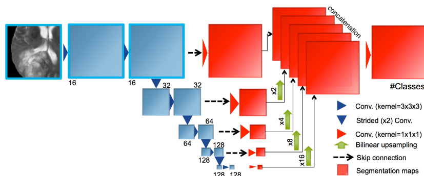
Fig. 4: Schematic of one of the FCN architecture used in EMMA. Shown are number of feature maps per layer. All kernels and feature maps are 3D, even though not depicted for simplicity.
