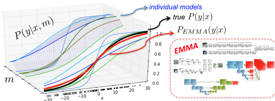
Fig. 2: Our ensemble of diverse networks, EMMA (red), averages out the bias infused by individual model configurations m , to approximate more reliably the true posterior (black), while being robust to suboptimal configurations. Posteriors on the left were obtained from multiple perceptrons, trained to classify clusters centred on 10 and -10 as a toy example, with different losses, regularizations and noise in the training labels. Their ensemble provides reliable estimates.
