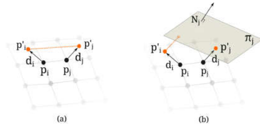
Figure 4 (a) In plane regularization term: the dotted line represents the distance used in F_1 , i.e. the distance between the points assuming they are coplanar. (b) Plane structure regularization term: the dotted line represents the distance between one of the control points and the plane corresponding to the other one. This information is used to compute the term F_2 .
